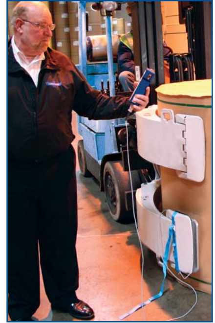
With Clamp Force Tester placed between load and the contact pad, technician is able to review and adjust clamp force easily.
